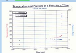
Fig 5. HOAt
