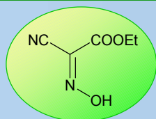
Figure 1. Structure of oxyma pure
